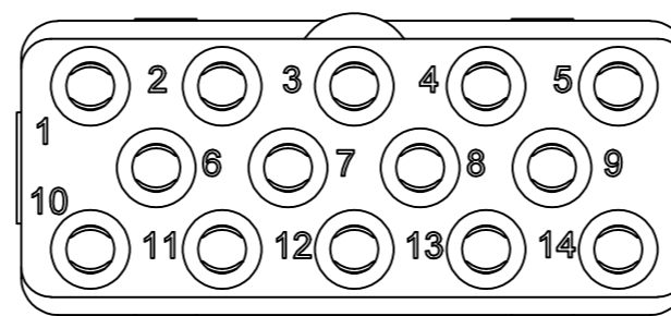
MATING FACE
