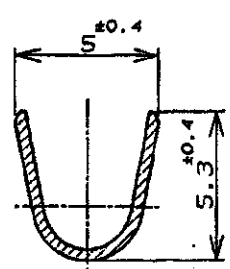
断面 "C"- "C" SECT
