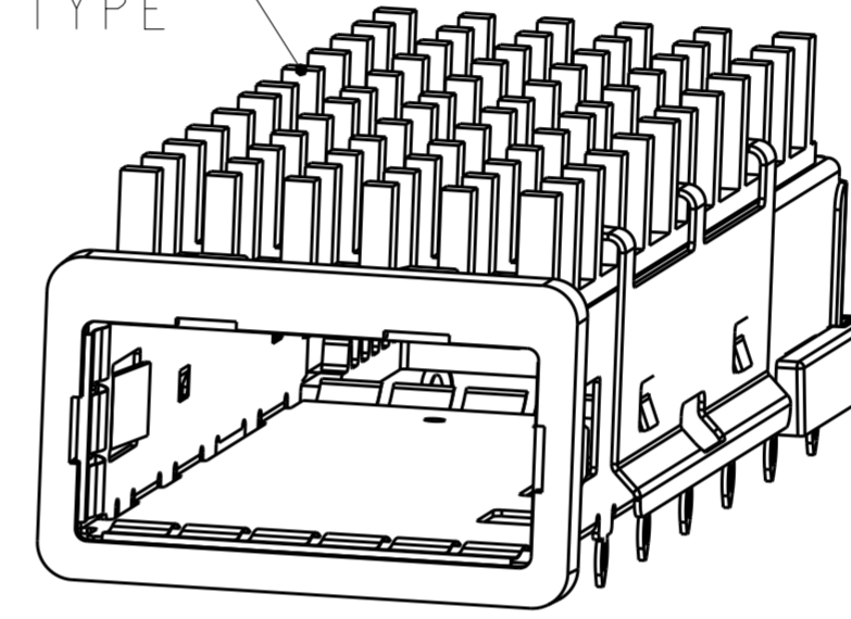
1888481-1, -2, -3 SCALE 3:1
