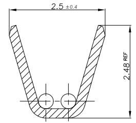
SECTION "A-A" Scale 20/1
