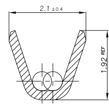
SECTION "B-B" Scale 20/1
