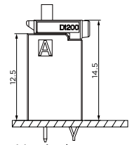
Vertical type
