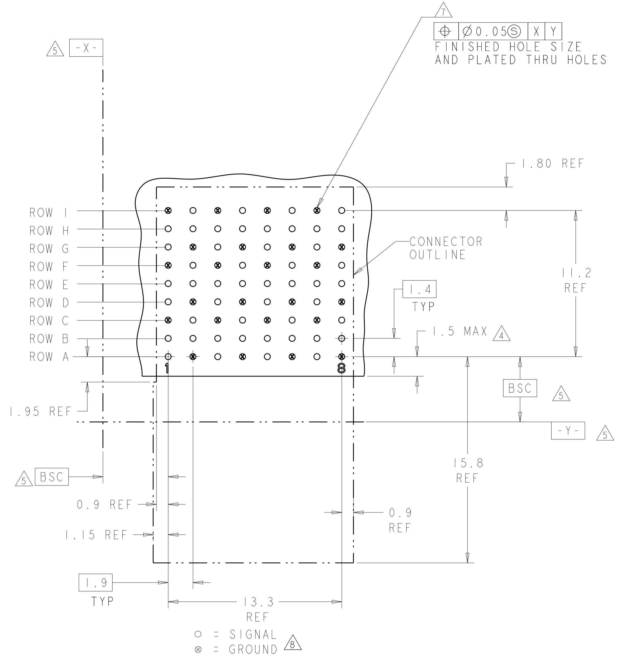
RECOMMENDED PC BOARD LAYOUT COMPONENT SIDE SHOWN
