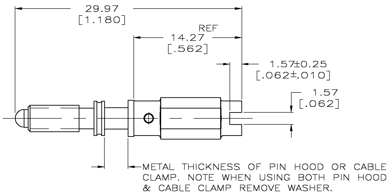
ASSEMBLED VIEW
