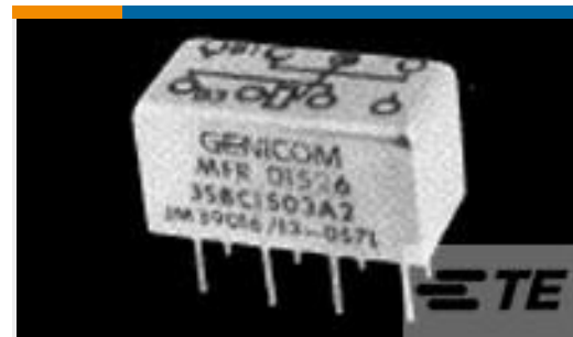
TE Part #2-1617072-6 3SBC1517A2 = M39016/13-056M
