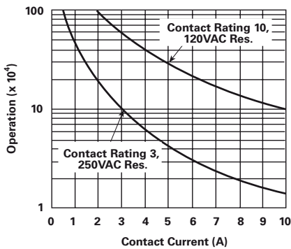
Electrical endurance
