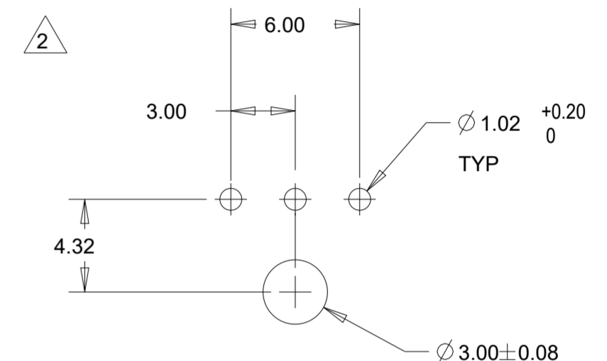
PCB LAYOUT FOR 3 POSITION COMPONENT SIDE
