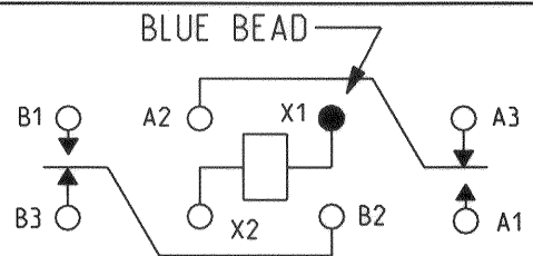
TERMINAL VIEW
