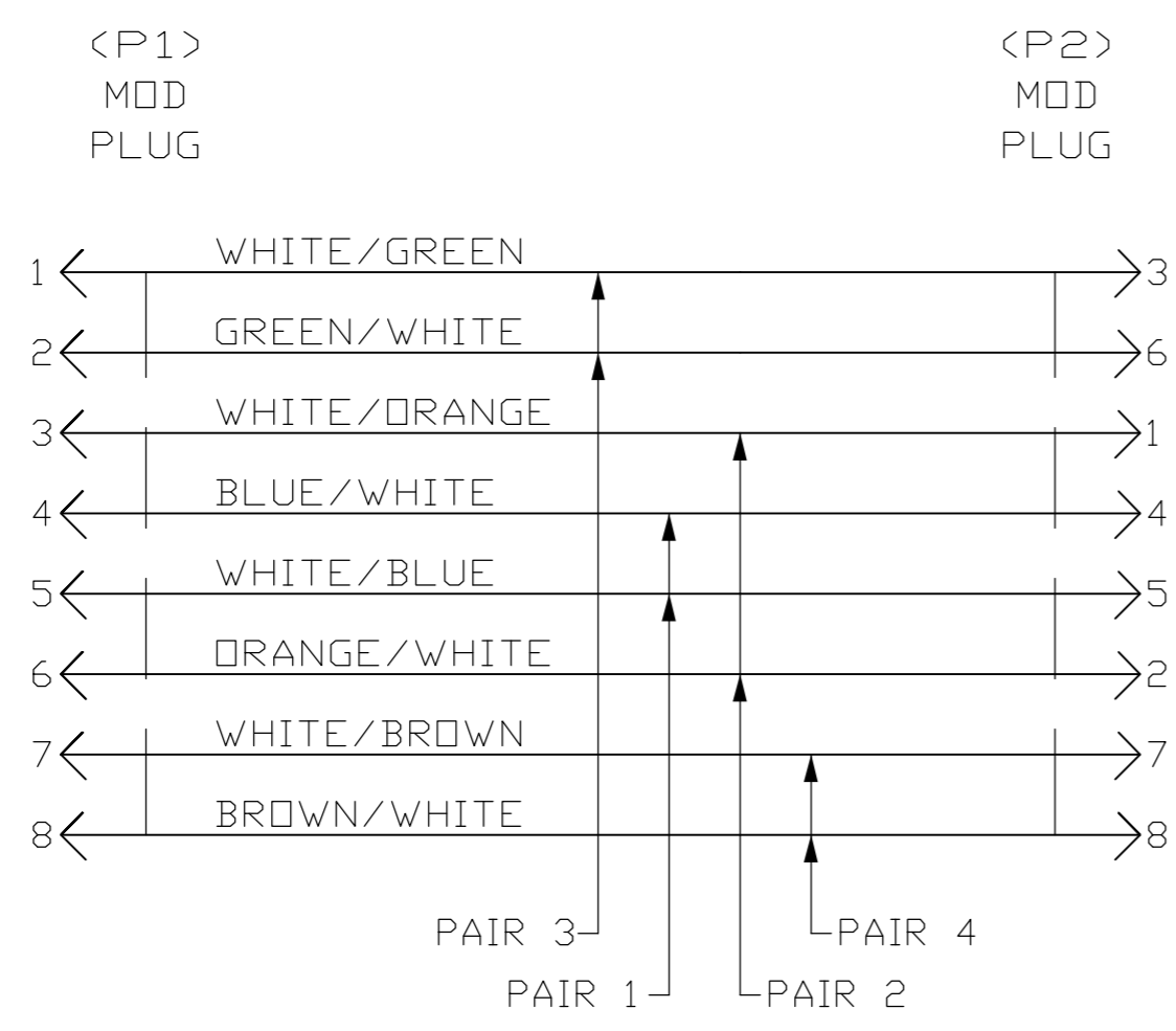
WIRING DIAGRAM CROSSOVER LAN TO 10 BASE T
