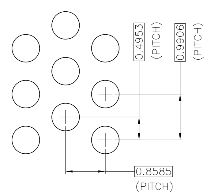
DETAIL N(20:1)
