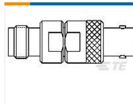
TE Part #1057845-1 3180 2320 00
