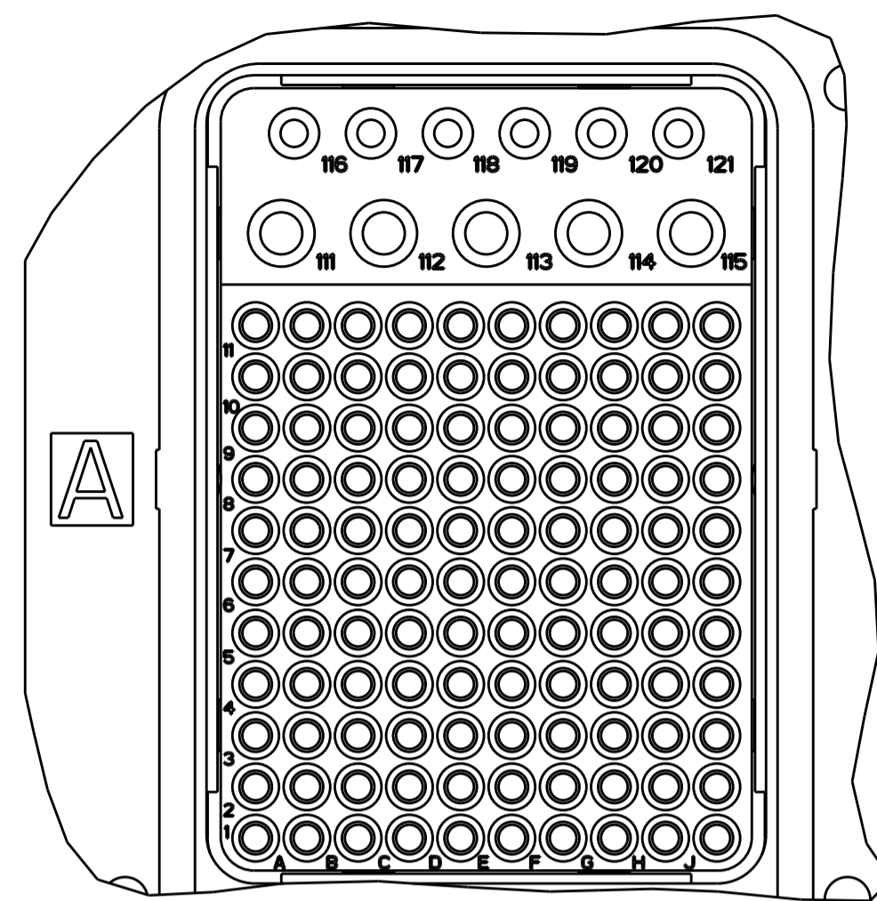
DETAIL A SCALE 3:1
