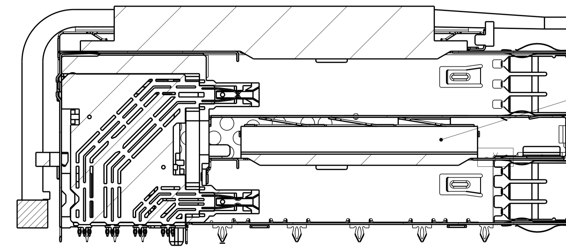
2299940-5 WITH LONGER INTERNAL HEAT SINK SECTION U-U SCALE 3:1
