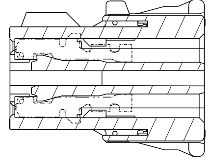
端子挿入状態 TERMINALS INSERTED CONDITION
