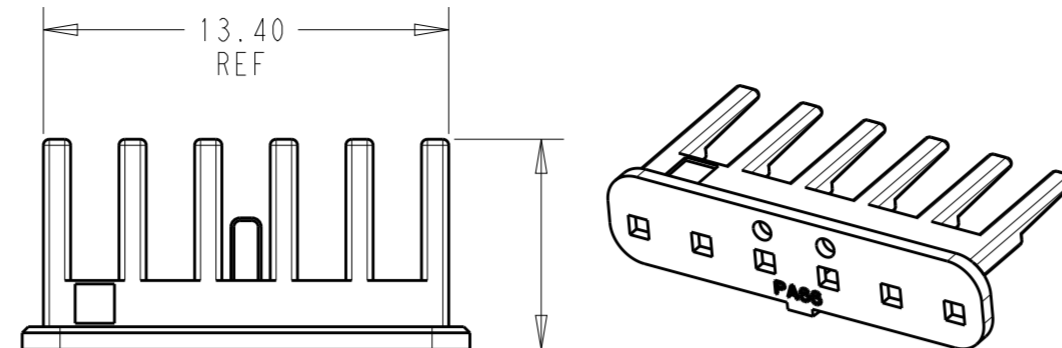
1x6 POSITION
