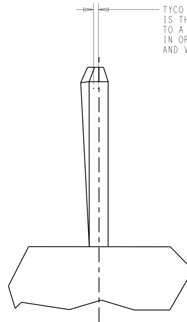
MATING TAB
