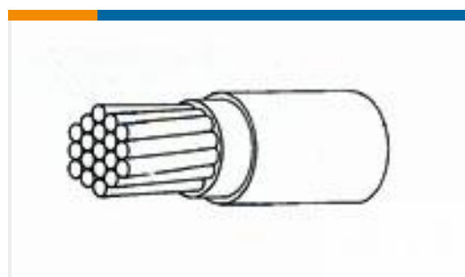
TE Part #218204-001 22759/34-20-9
