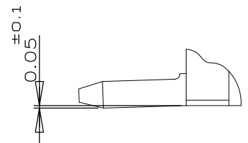
DETAIL E SCALE 10-1
