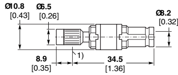
Part No. 2-1393670-3 ♦ Coupling Type A, B 2 , F 2
