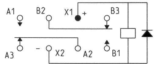
TERMINAL VIEW
