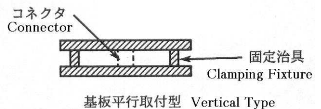
Fig.5 コネクタ固定方法 Method of Connector Mounting for Vibration and shock
