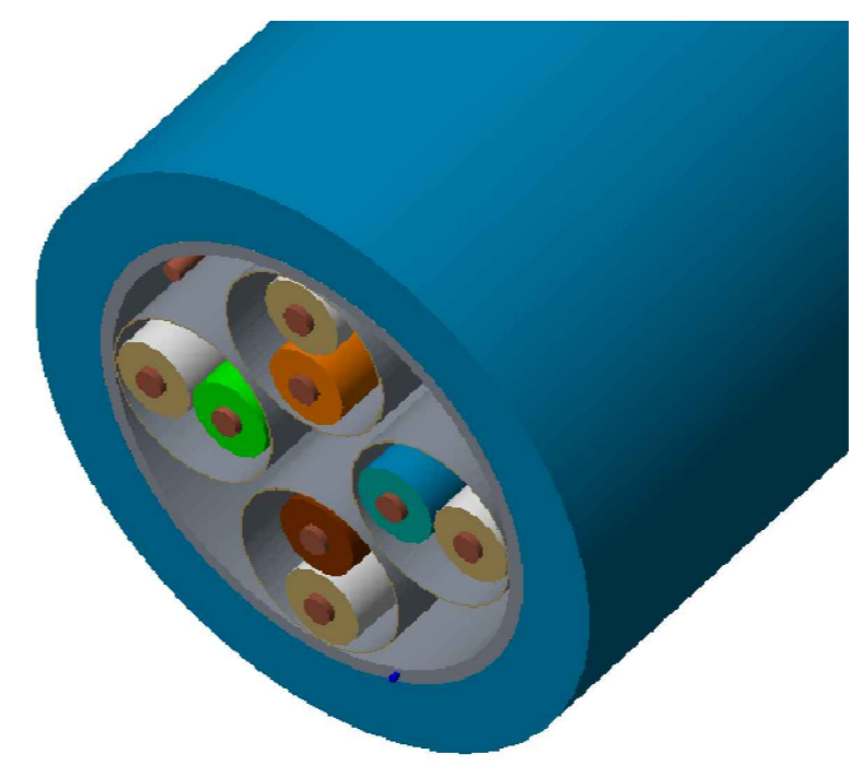
SECTIONAL ISO VIEW OF THE CABLE
