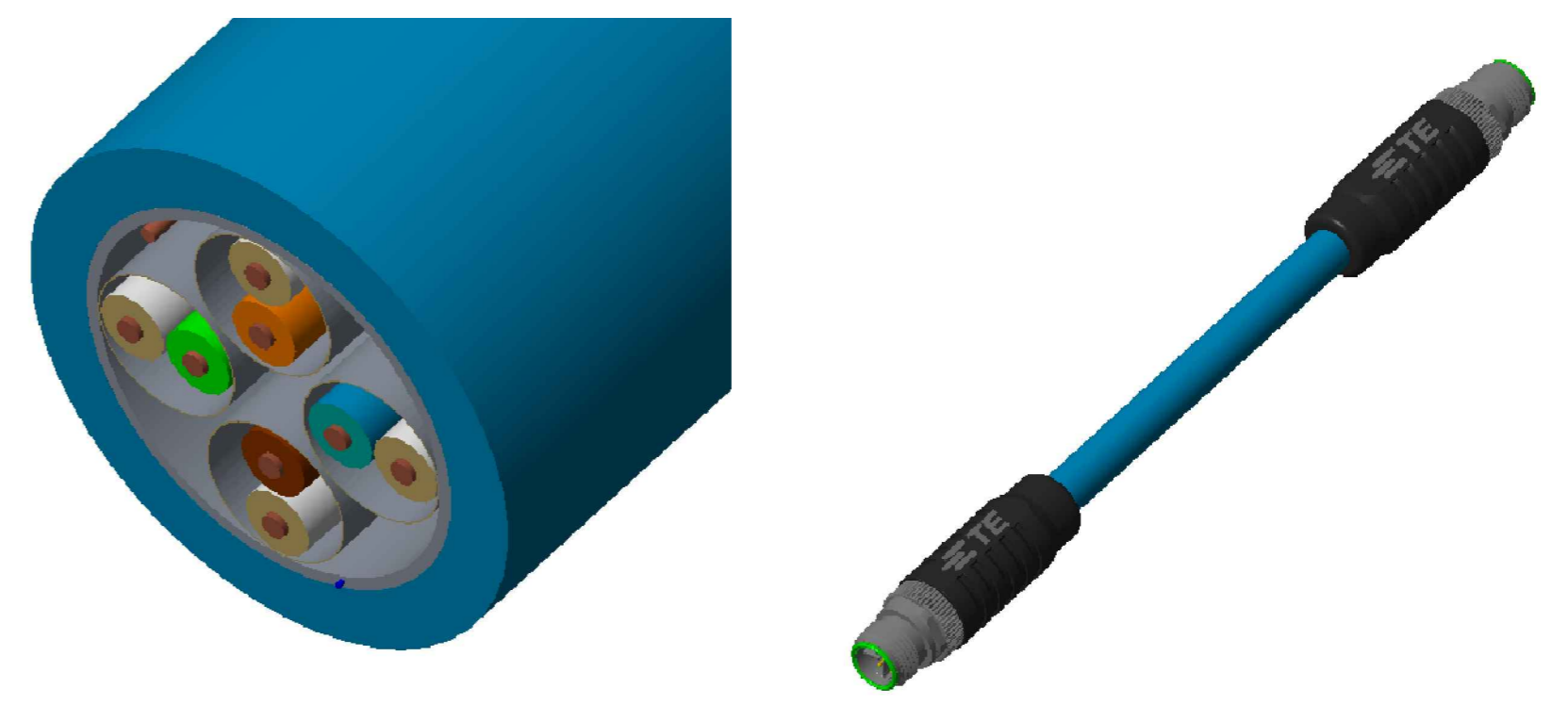
SECTIONAL ISO VIEW OF THE CABLE
