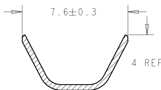
SECTION D-D SCALE 6:1
