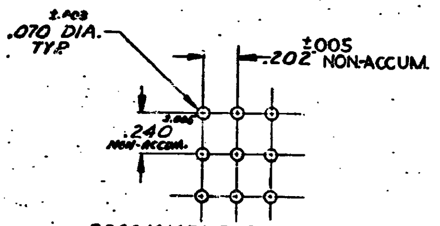
RECOMMENDED LAYOUT FOR .125 THICK P.C. BOARD
