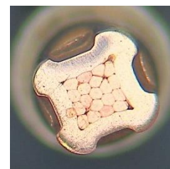
Crimp Too Loose and Void on Within Crimp
