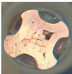
Crimp Too Loose and Voids in the Crimp
