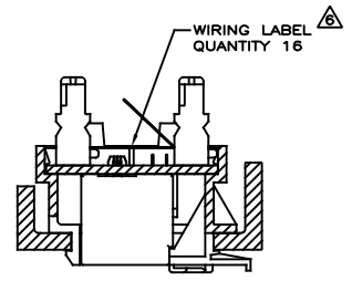
SECTION B-B ROTATED 90° CCW SCALE 2:1
