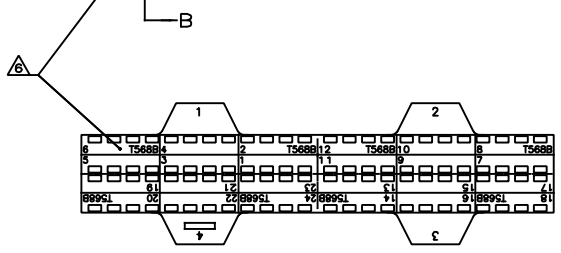
T568B SIDE 110 CONNECTOR UNIVERSAL WIRING LABELS
