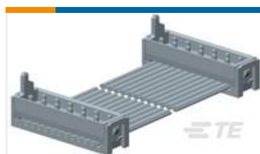
TE Part #1483354-2 MICRO-MATCH LEAD 12P 150MM
