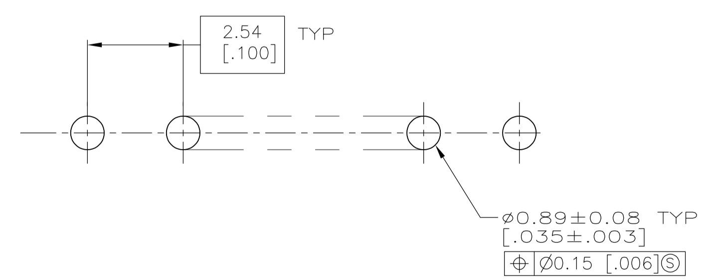
RECOMMENDED BOARD LAYOUT
