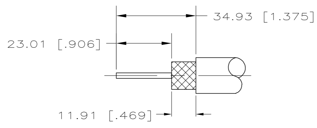
DETAIL B
