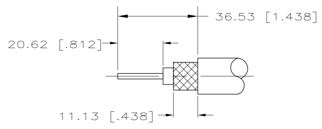
DETAIL A
