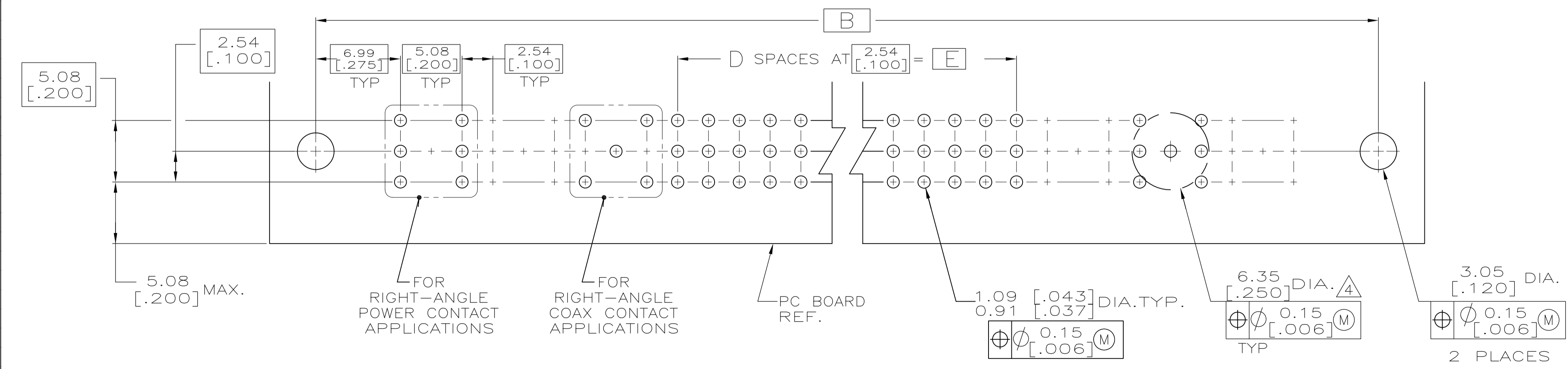
RECOMMENDED PC BOARD LAYOUT △
