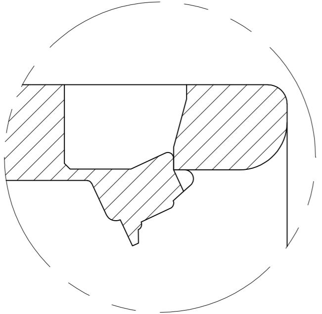
5 DETAIL A LATCH POSITION AFTER CRIMPING SCALE 10:1
