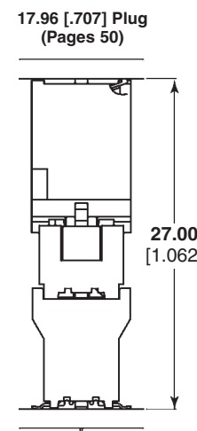
17.96 [.707] Plug (Pages 50) Raised Receptacle (Pages 58 and 59)
