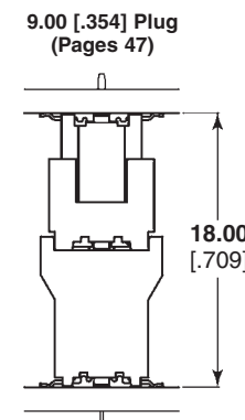
9.00 [.354] Plug (Pages 47) Raised Receptacle (Pages 58 and 59)
