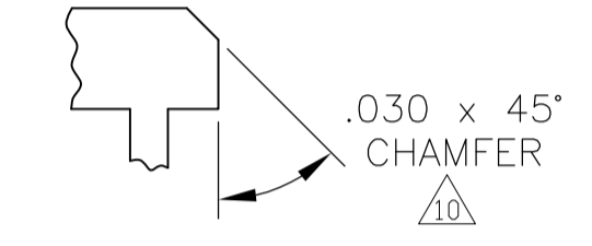
DETAIL X SCALE 5:1
