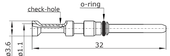
Main Dimensions contact pin
