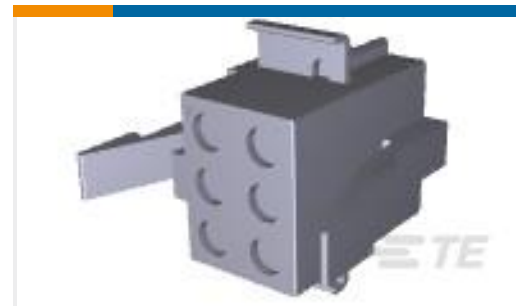
TE Part #1-480690-0 06P CMNL PLUG HSG D/L PM NAT
