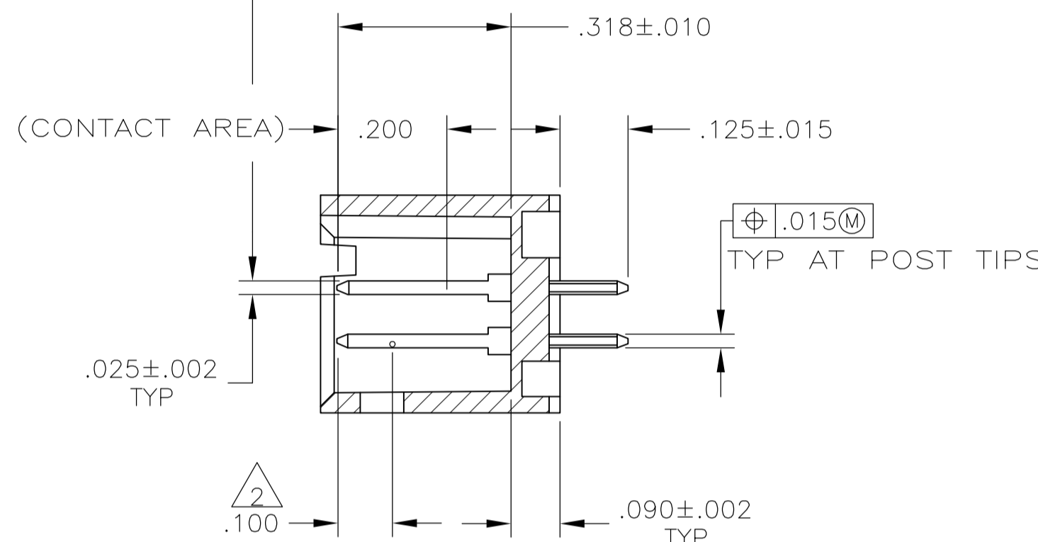
SECTION X-X
