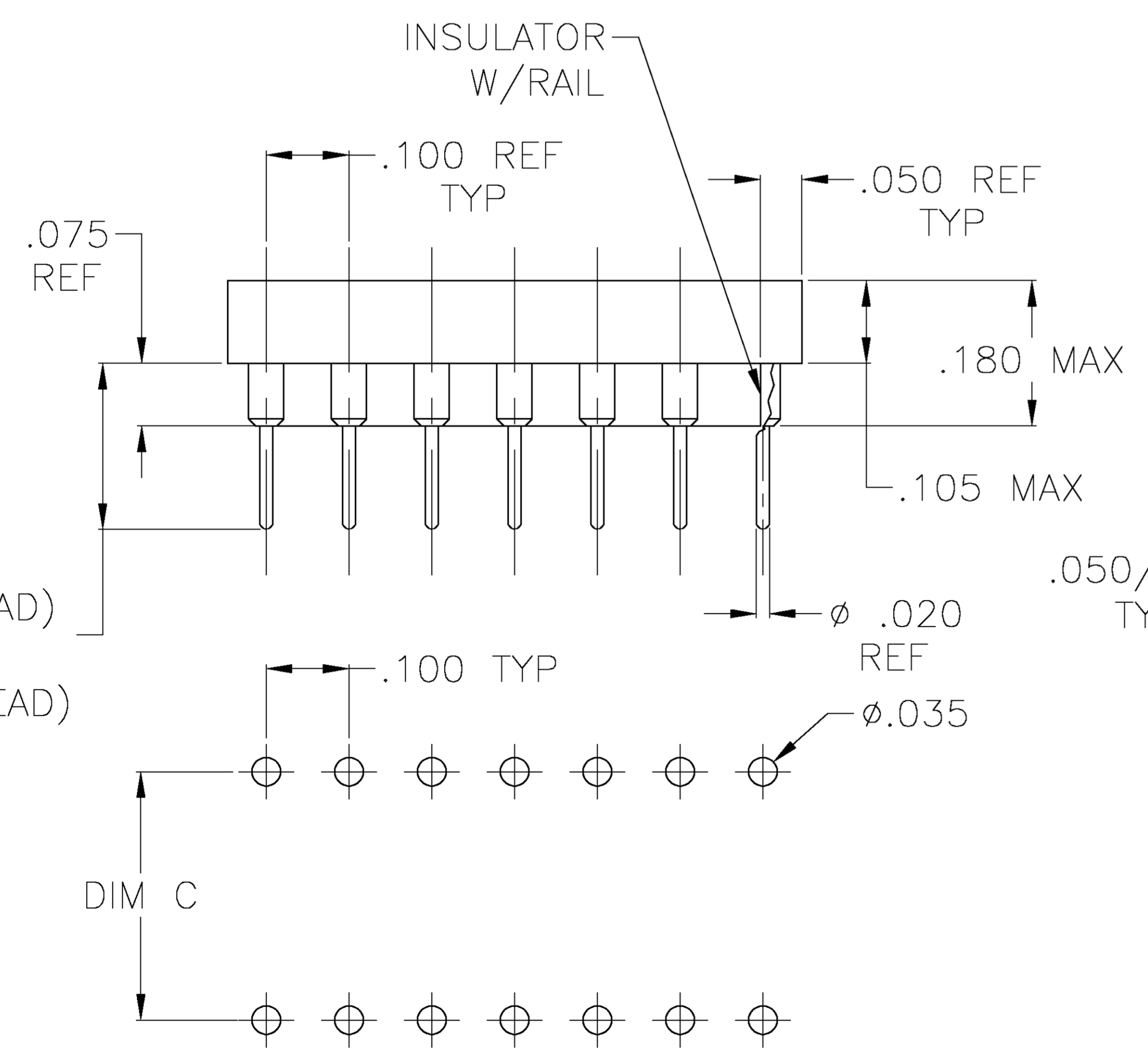
P.C.B. HOLE LAYOUT TOLERANCE ±.003
