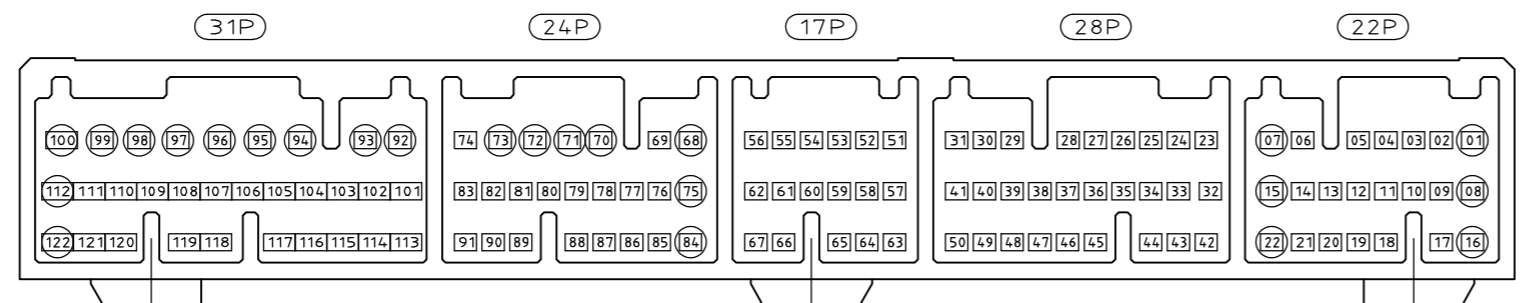
△ FIG 1 CIRCUIT NUMBERS △ 0.4φZ|Y|DTM (FOR POWER CIRCUIT)
