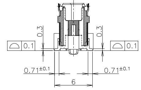
SECT. Y-Y (GROUND POSITION)
