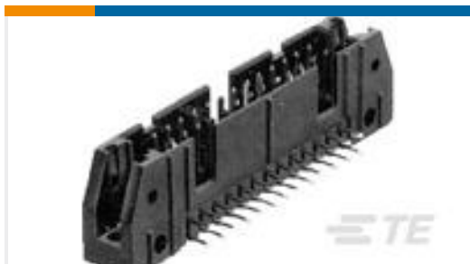
TE Part #207612-7 SKT HDR ASSY, 10 P, MMATE LF
