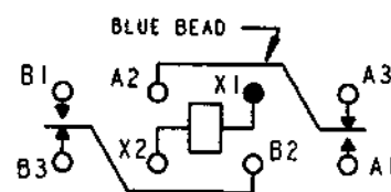
TERMINAL VIEW
