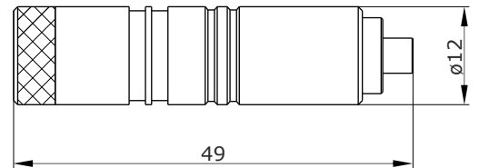
Main Dimensions positioning insert
