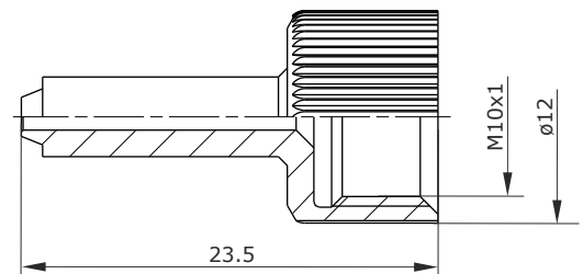
Main Dimensions removing sleeve
