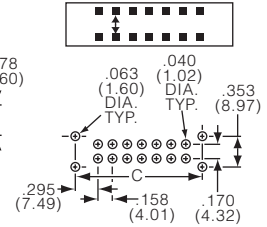
CONTACT ARRANGEMENT
