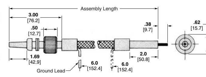
Part Number 846938
