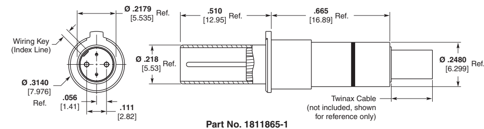
Part No. 1811865-1
