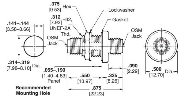
Outline 2
