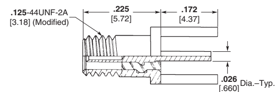
Straight Printed Circuit Receptacle* Part No. 141-0004-0001
