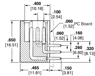
Part Number 204818-4
