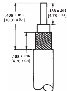
Recommended Strip Length
