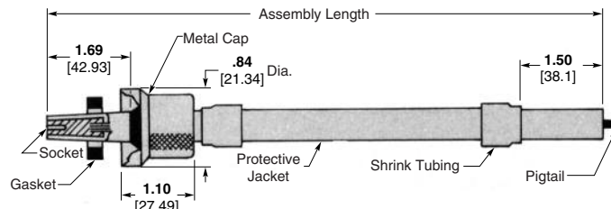
Part Number 861813
