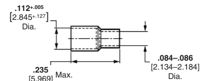
Ferrule Part Number 1-332057-0
