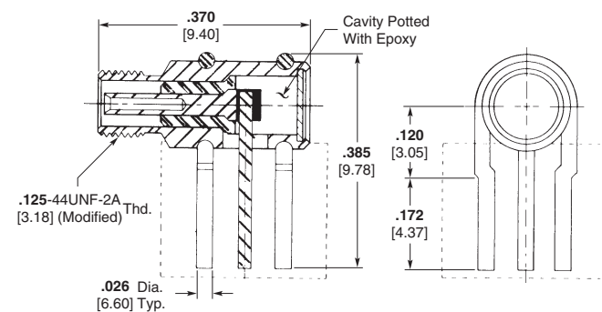
Right-Angle Printed Circuit Receptacle* (Standard Mounting Pattern) Part Number 141-0010-0001
