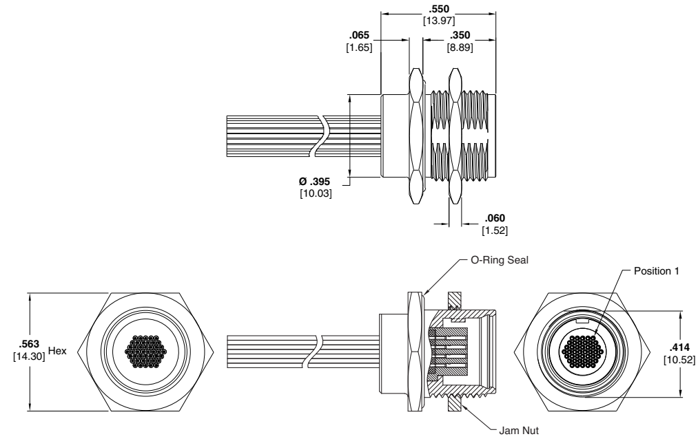
44 Position Drawing Number 1589062
