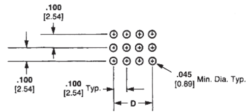
Right-Angle Wrap-Type Posted Contacts
