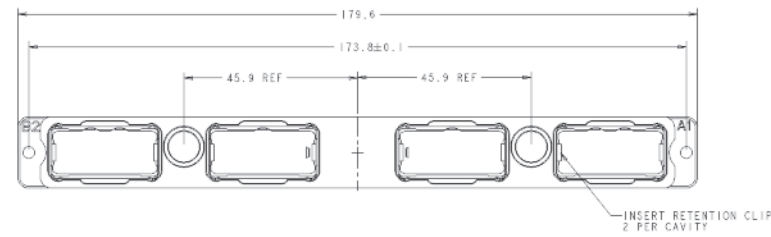
Receptacle, w/(2) thru holes 1996487-1
