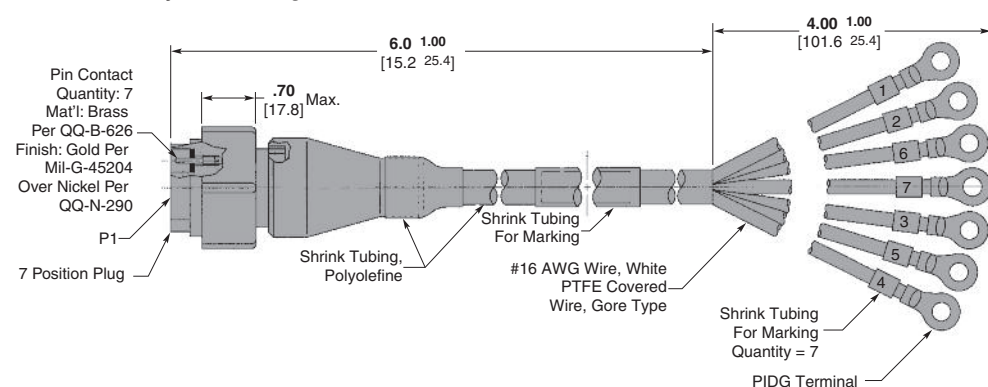
Part Number 447288-1
