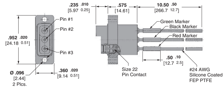
Part Number 443815-1
