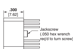
Plug
