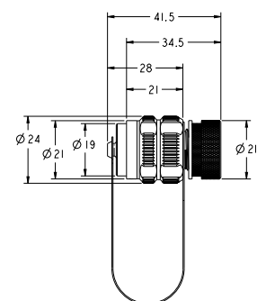
38999 Plug Shell Kit for mini EB
