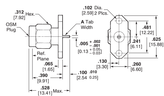
Outline 3
