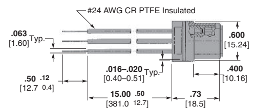
Part Number 867761-1
