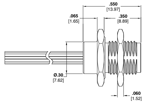
7 Position Drawing Number 1589060
