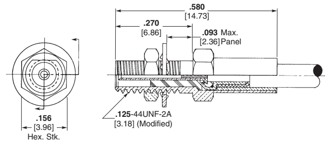
Bulkhead Jack 1
