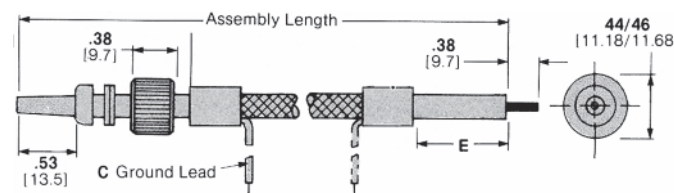
Part Number 846985
