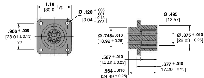
Part Number 449652-1
