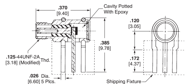
Right-Angle Printed Circuit Receptacle* (Small Mounting Pattern) Part Number 141-0019-0001
