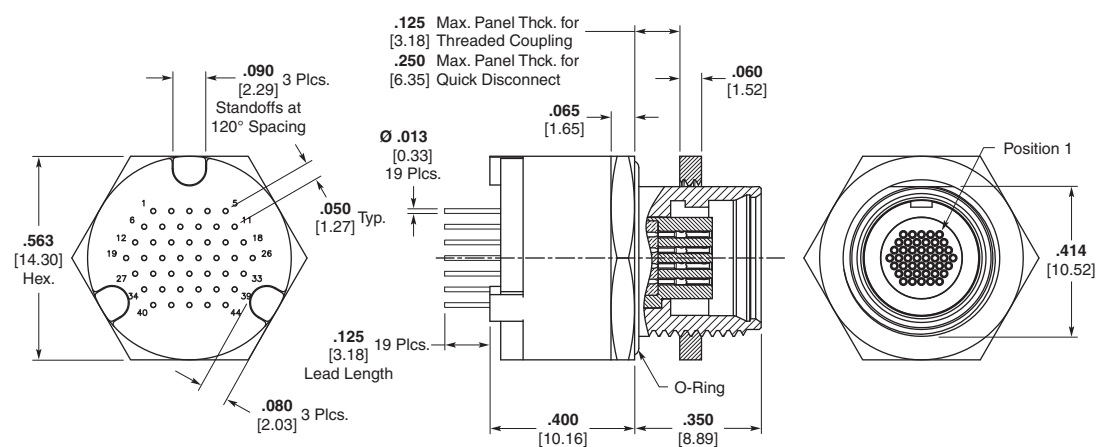
Receptacle Assembly 44 Position Drawing Number 1589955
