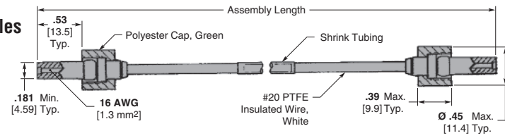
Part Number 860529
