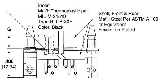
9 Position (with Locking Post)
