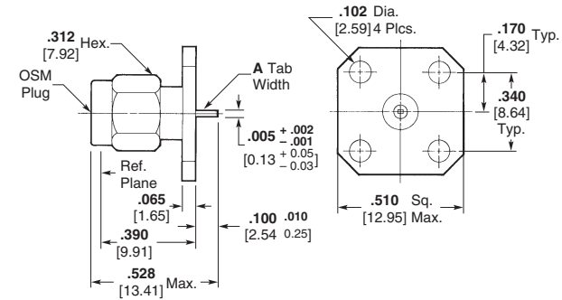
Outline 4
