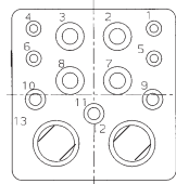
13CQ2 2, 3 4 Size 20 3 Size 16 4 Size 12 2 Size 8 Quadrax
