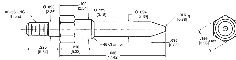
Part Number 447448-1
