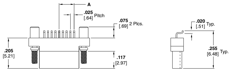
Jackscrews Omitted for Clarity
