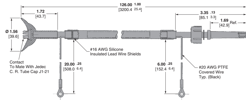
Part Number 867615-2
