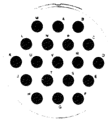
25-19 19 SIZE 12 CONTACTS
